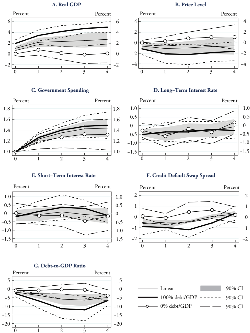
Chart A2 Blanchard-Perotti Identification, Annual Frequency
