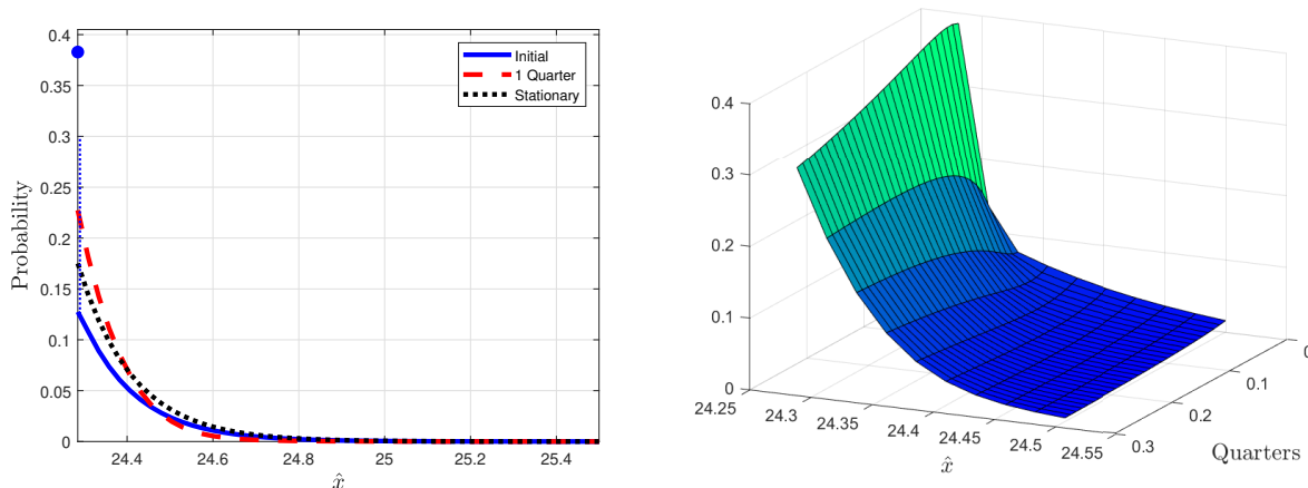
(a) Distribution on Impact and After One Quarter
