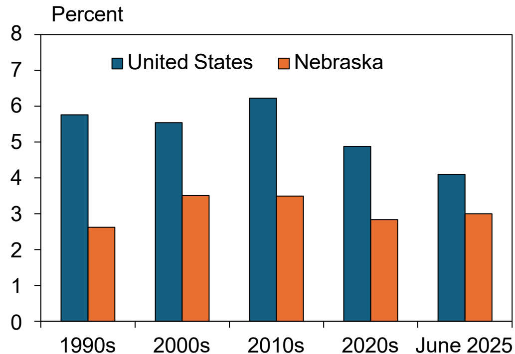
Unemployment Rate
