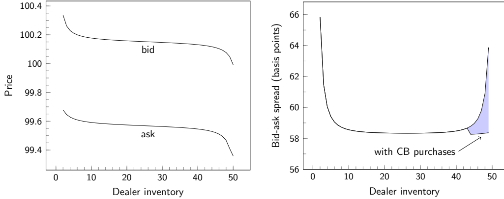
(a) Bid and ask prices for an isoelastic model. Buyer elasticity is \gamma = 400 . Seller elasticity is \nu = 300 . The trade-rate constants are c = 100,000 and k = 50,000 . The discount rate is r = 0.1 . The bond dividend rate is d(x) = 0.1x , implying a perfect-markets bond price of 0.1/r = 1 . The prices shown are scaled by 100.
