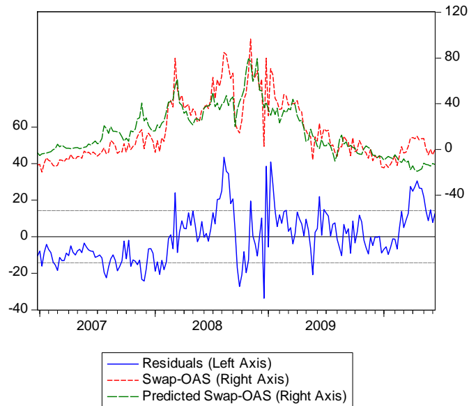
Figure 2. Swap OAS: Predicted, Actual and Residual
