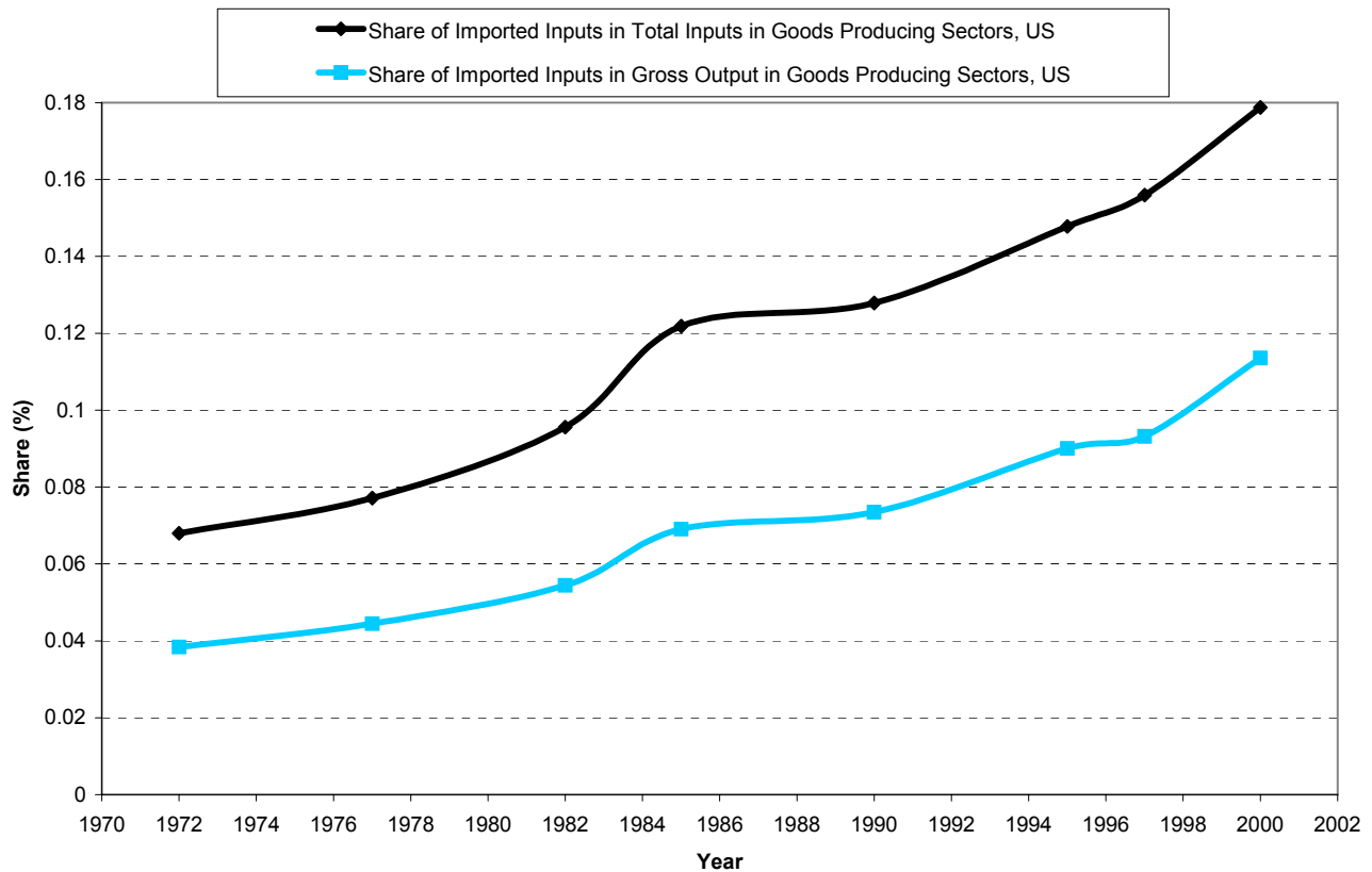
Figure 1: Imported Inputs
